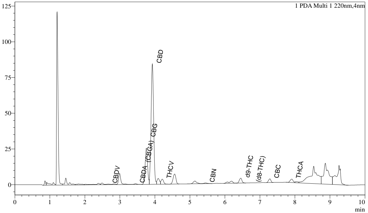
Chromatogram
